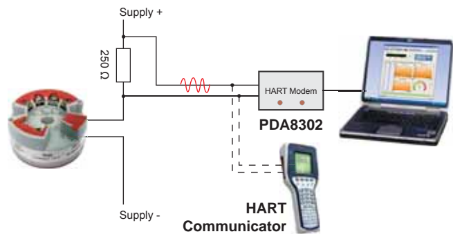
PD302 HART Programming
