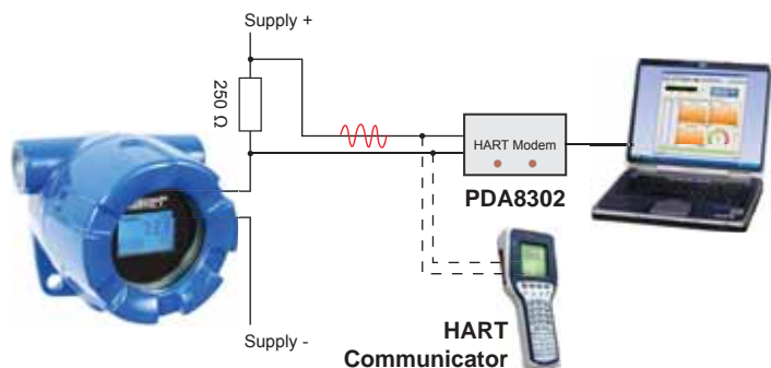
PD310 & PD312 HART Programming
