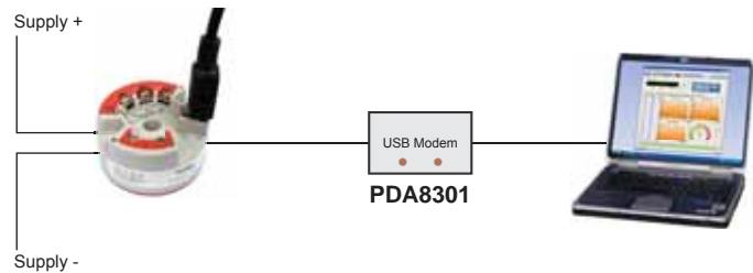
PD301-PD306 PC Programming
