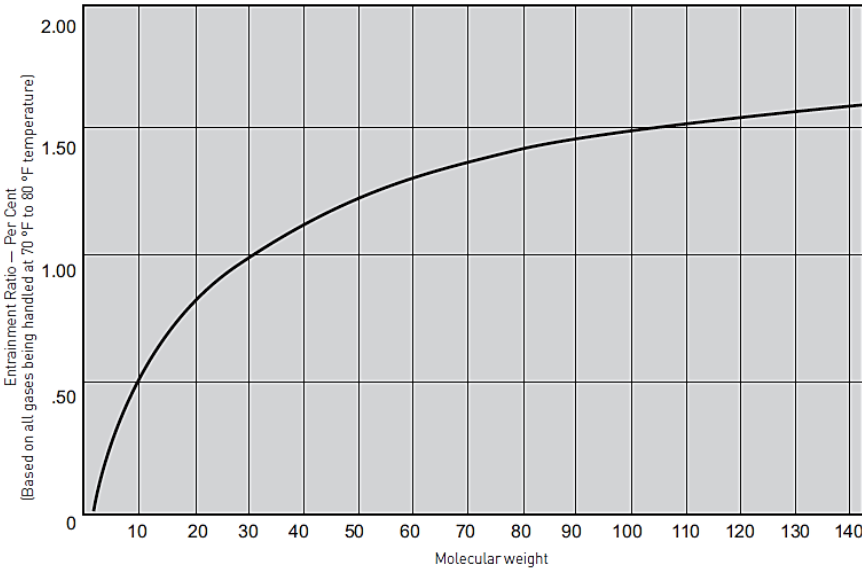
MOLECULAR WEIGHT ENTRAINMENT RATIO CURVE (NO. 1)*
